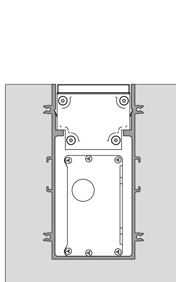
RECESSED BOX INSTALLATION
