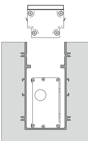
WALKABOUT GROUND INSERTION
