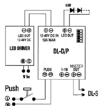
Schema/wiring Push 230Vac
