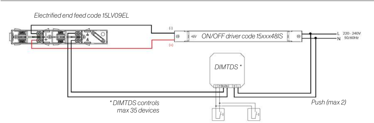
WIRING DIAGRAM LV-TRACK FOR SWITCH DIM
