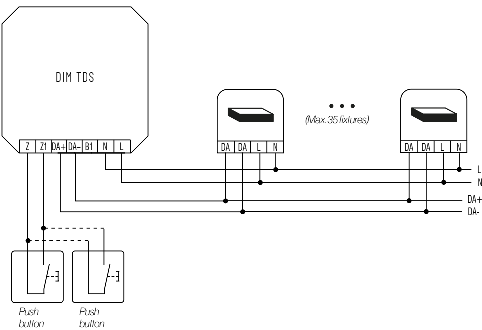
CONNECTION DIAGRAM
