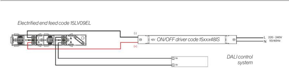
WIRING DIAGRAM LV-TRACK FOR DALI
