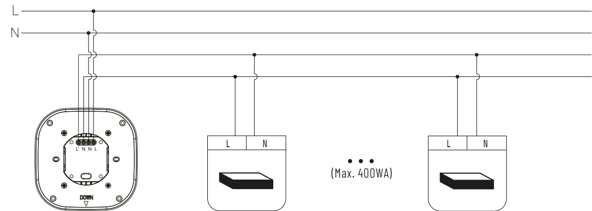
CONNECTION DIAGRAM
