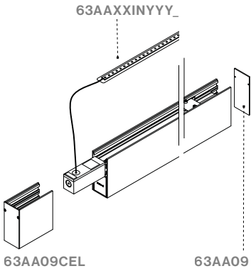
EXAMPLE OF MAKROT PRO CONFIGURATION ON EUROSTANDARD THREE-PHASE TRACK
