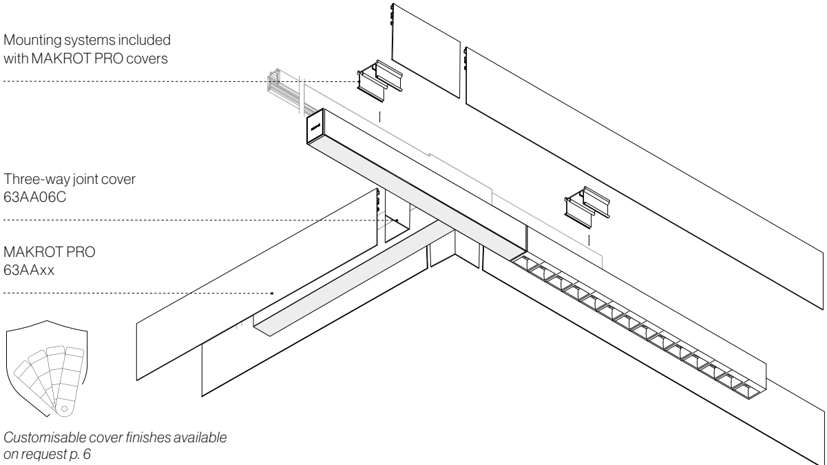
EXAMPLE OF MAKROT PRO CONFIGURATION ON EUROSTANDARD THREE-PHASE TRACK
